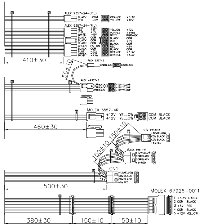
OUTPUT WIRE
